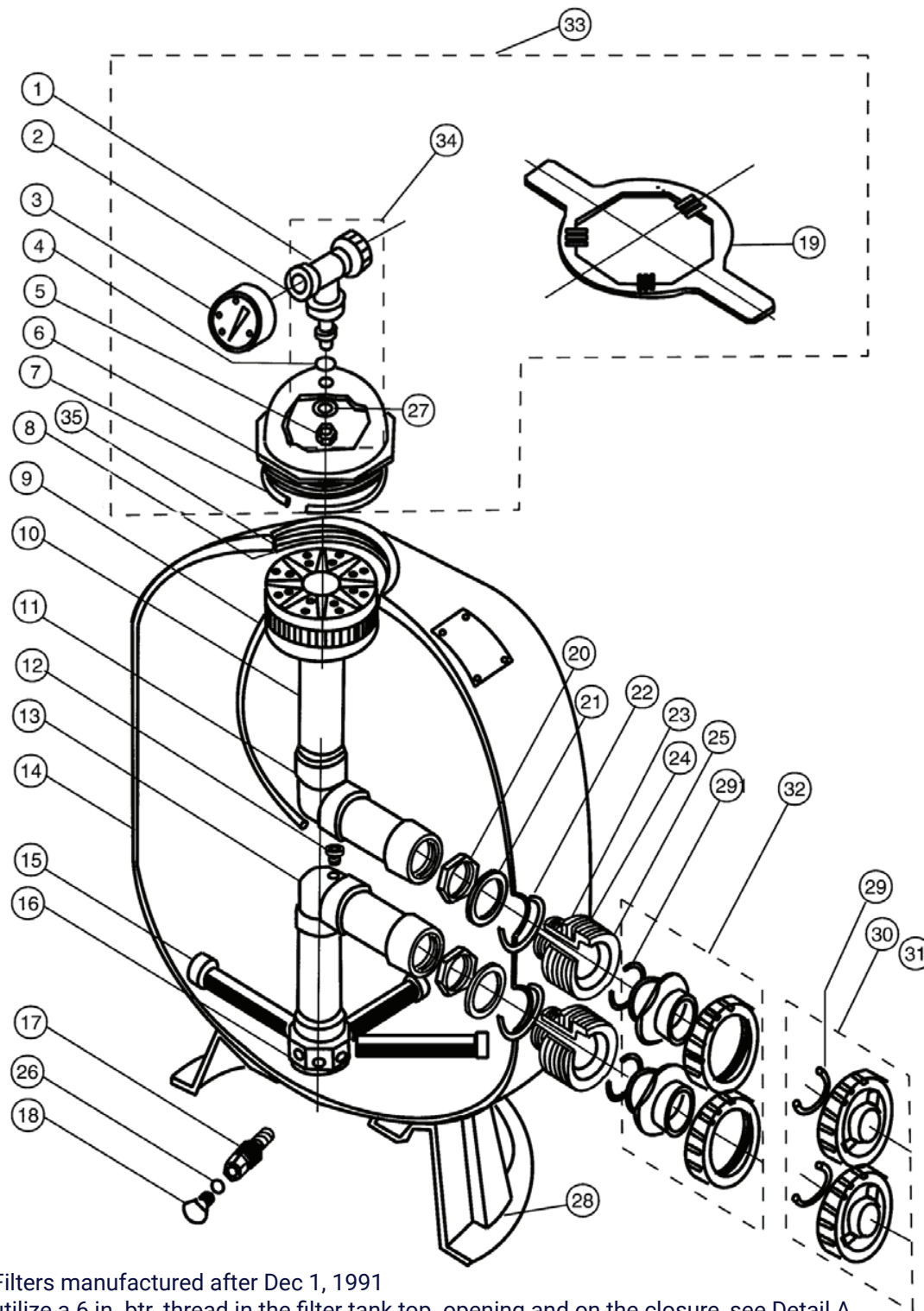
Detail A after 12/1/91 6 in. btr. Thread.
